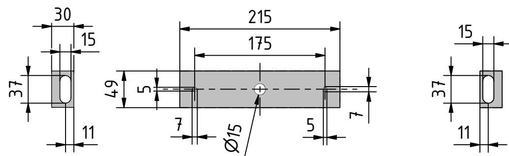
Adapter 20
